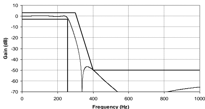
Figure 18 Low Pass Sub-Audio Band Filter for CTCSS and DCS
