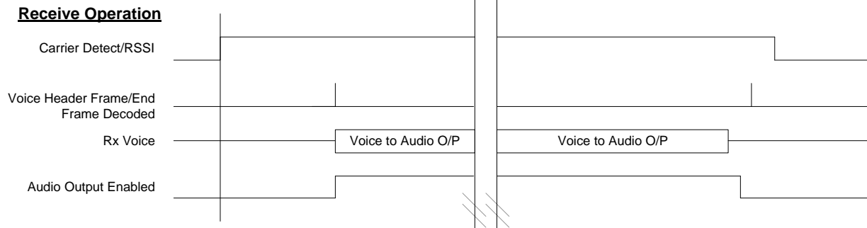
Figure 8 Typical Timing for PTT Delay
