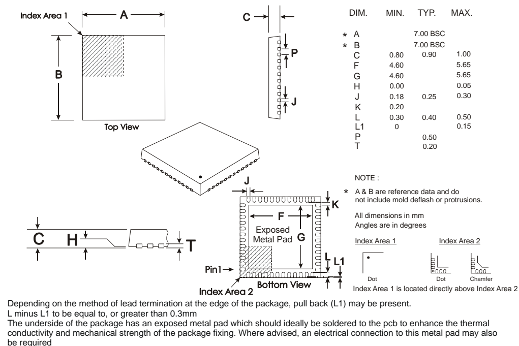
Figure 14 48-pin VQFN Mechanical Outline (Q3)
