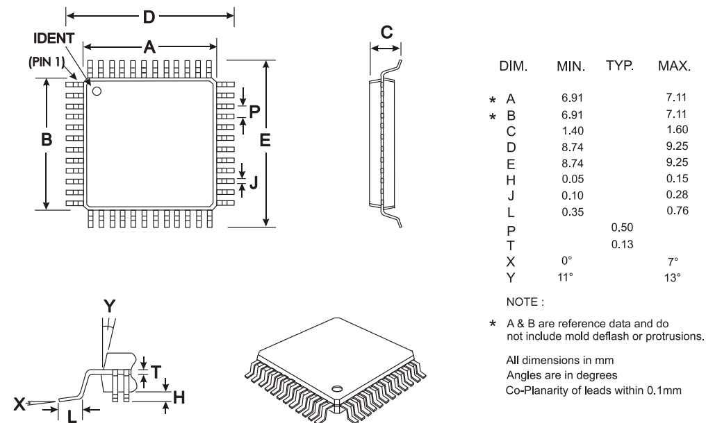
Figure 13 48-pin LQFP Mechanical Outline (L4)
