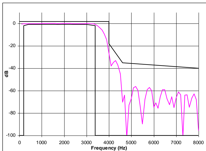
Figure 11 ADC Input Filter - Typical Response
