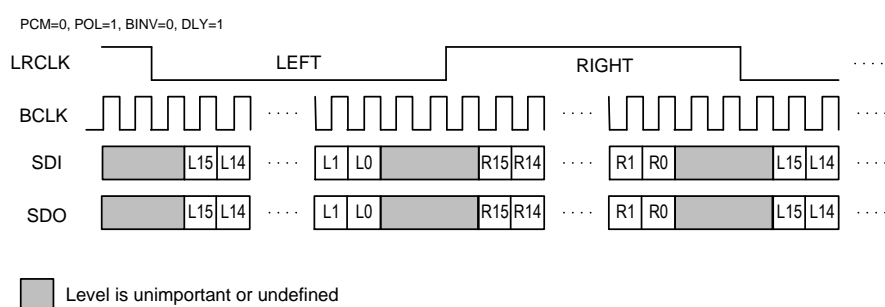
Figure 35 I2S Mode Data Transfer
