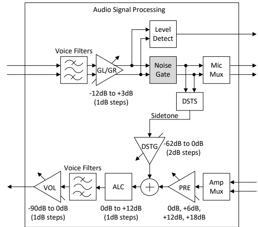
Figure 13 Audio signal processing block diagram with Noise Gate block highlighted
