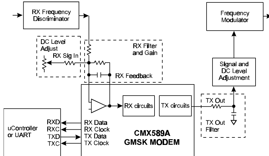
Figure 1: Block Diagram
