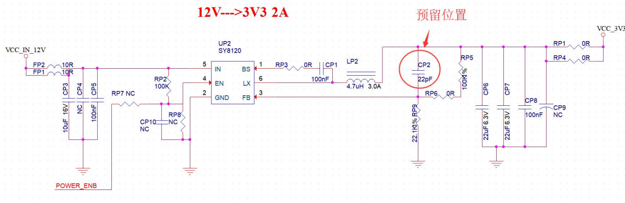
Figure 7 DC-DC reference design drawing
