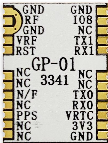
Figure 4 Pin diagram
