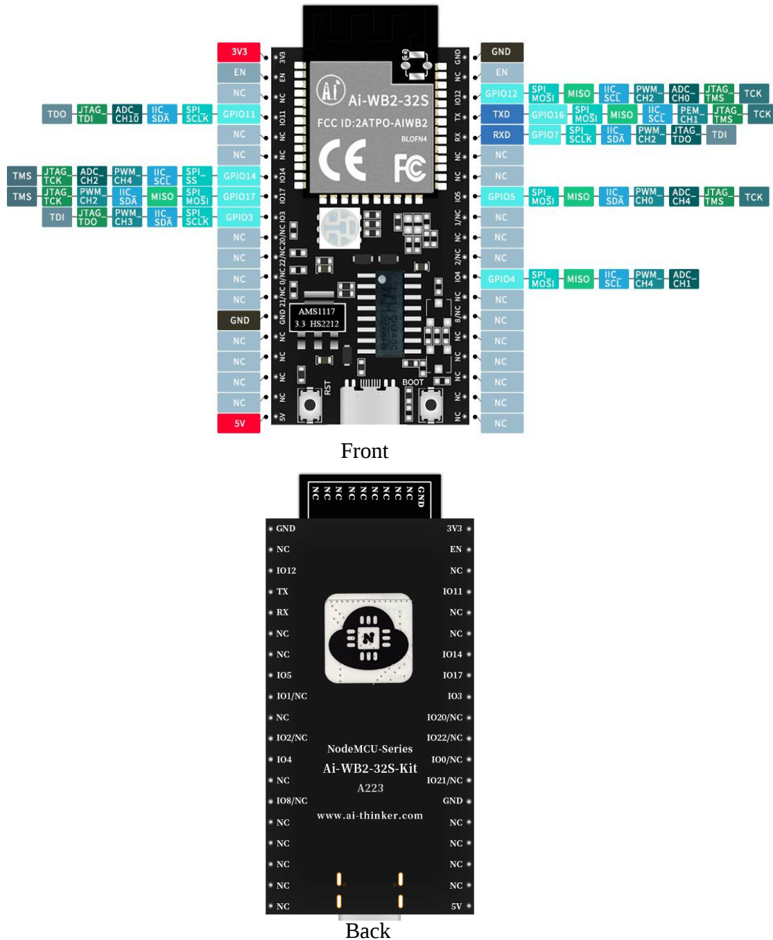
Figure 5 pin diagram
