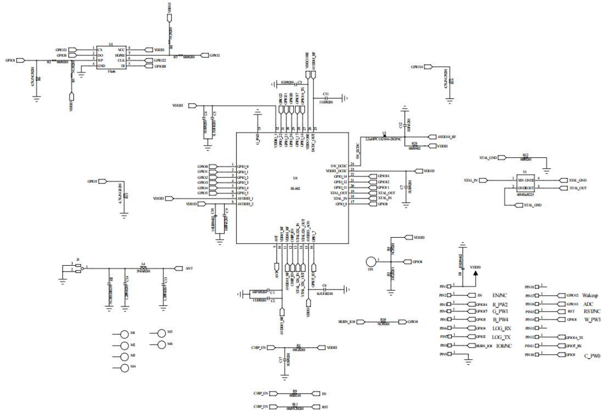
Figure 7 Module schematic
