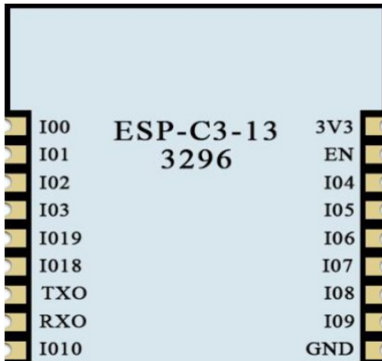
ESP-C3-13 Diagram of Pin
