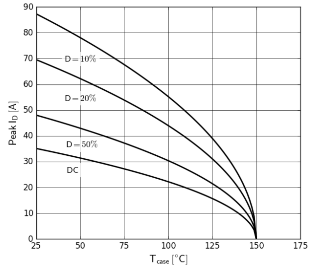
Figure 10. Current Derating Pulse width \leq 10\mu\text{s} , V_{GS} \geq 10V
