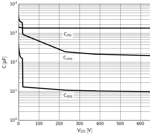
Figure 5. Typical Capacitance V_{GS}=0V , f=1\text{MHz}
