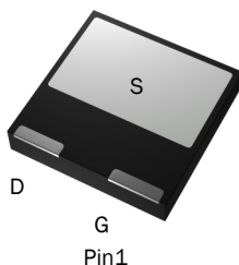
TP65H070G4LSG PQFN (bottom view)
