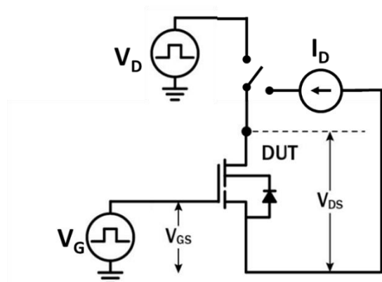
Figure 18. Dynamic R_{DS(on)eff} Test Circuit
