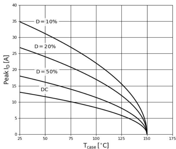
Figure 10. Current Derating
