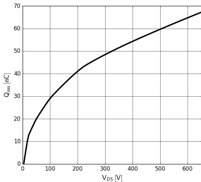
Figure 7. Typical Q_{OSS}
