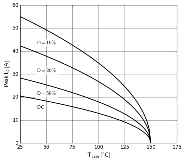
Figure 10. Current Derating
