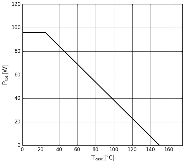
Figure 14. Power Dissipation
