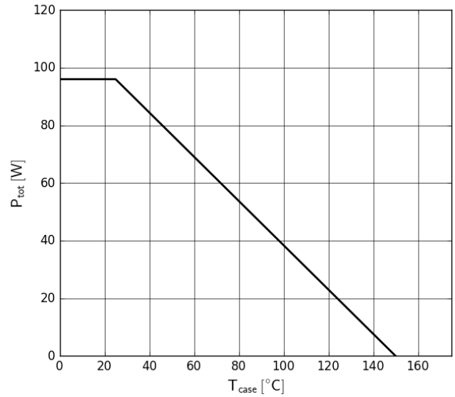
Figure 14. Power Dissipation
