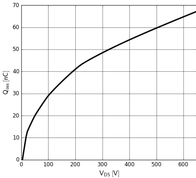
Figure 7. Typical Q_{OSS}
