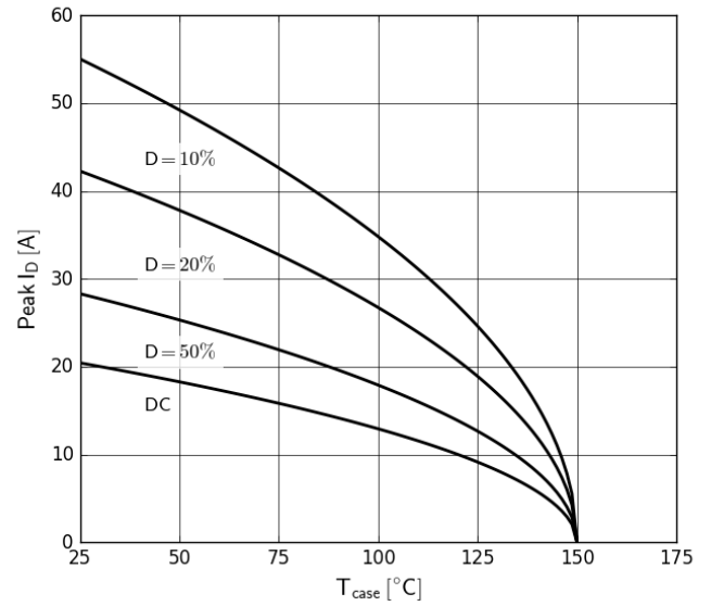
Figure 10. Current Derating
