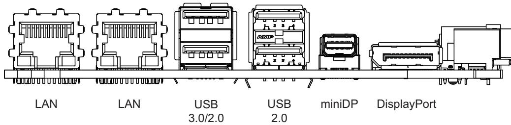
Figure 2: C0Me Ref. Carrier-i T10 TNI Rear Panel
