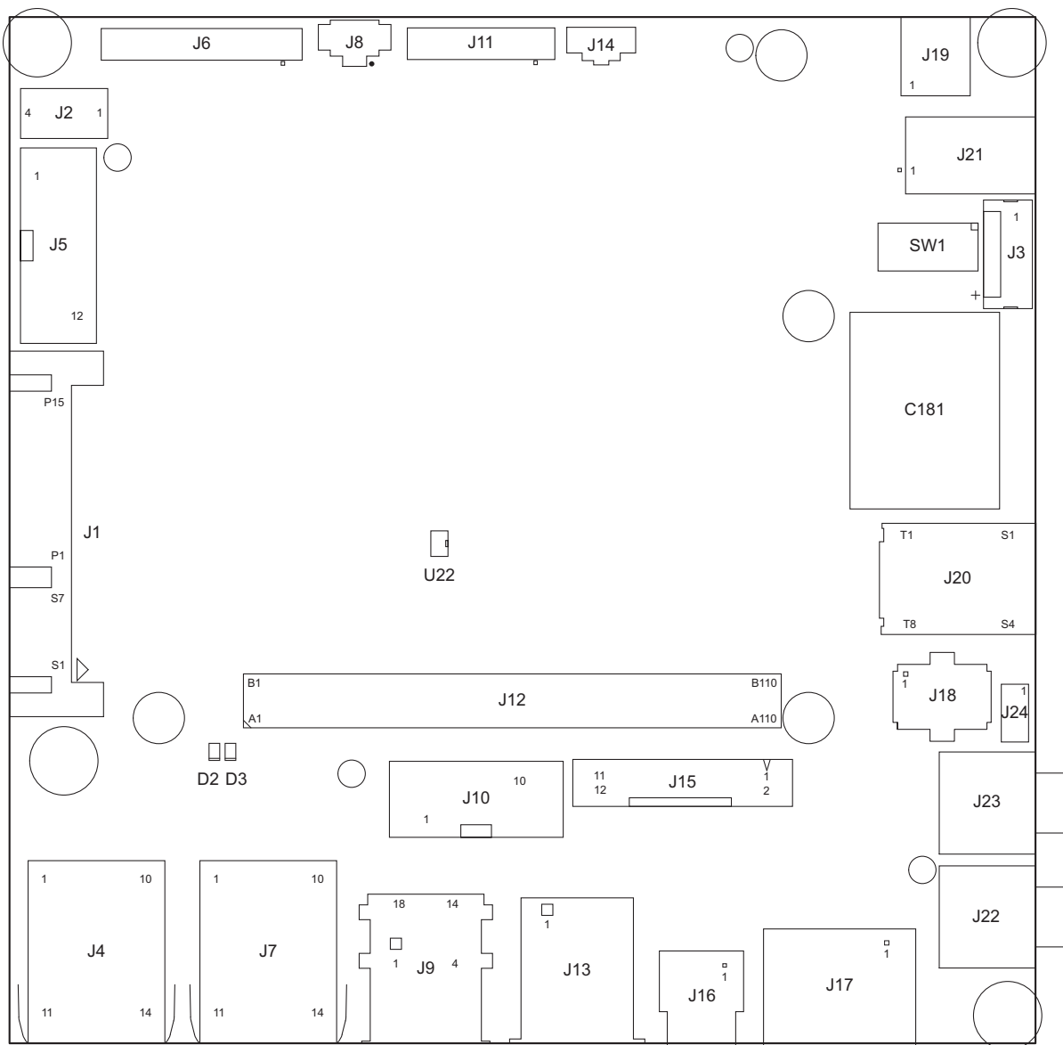
Figure 3: C0Me Ref. Carrier-i T10 TNI Layout - Top View
