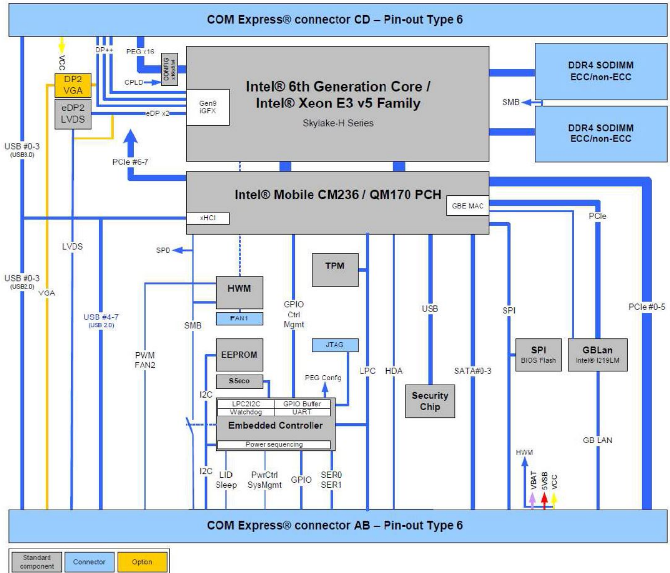
Figure 1: Block Diagram COMe-bSL6
