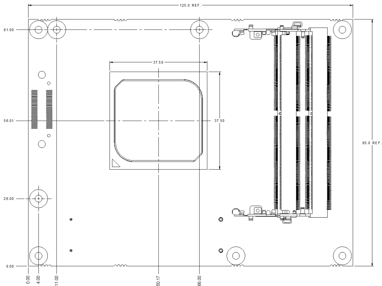
Figure 7: Module Dimensions
