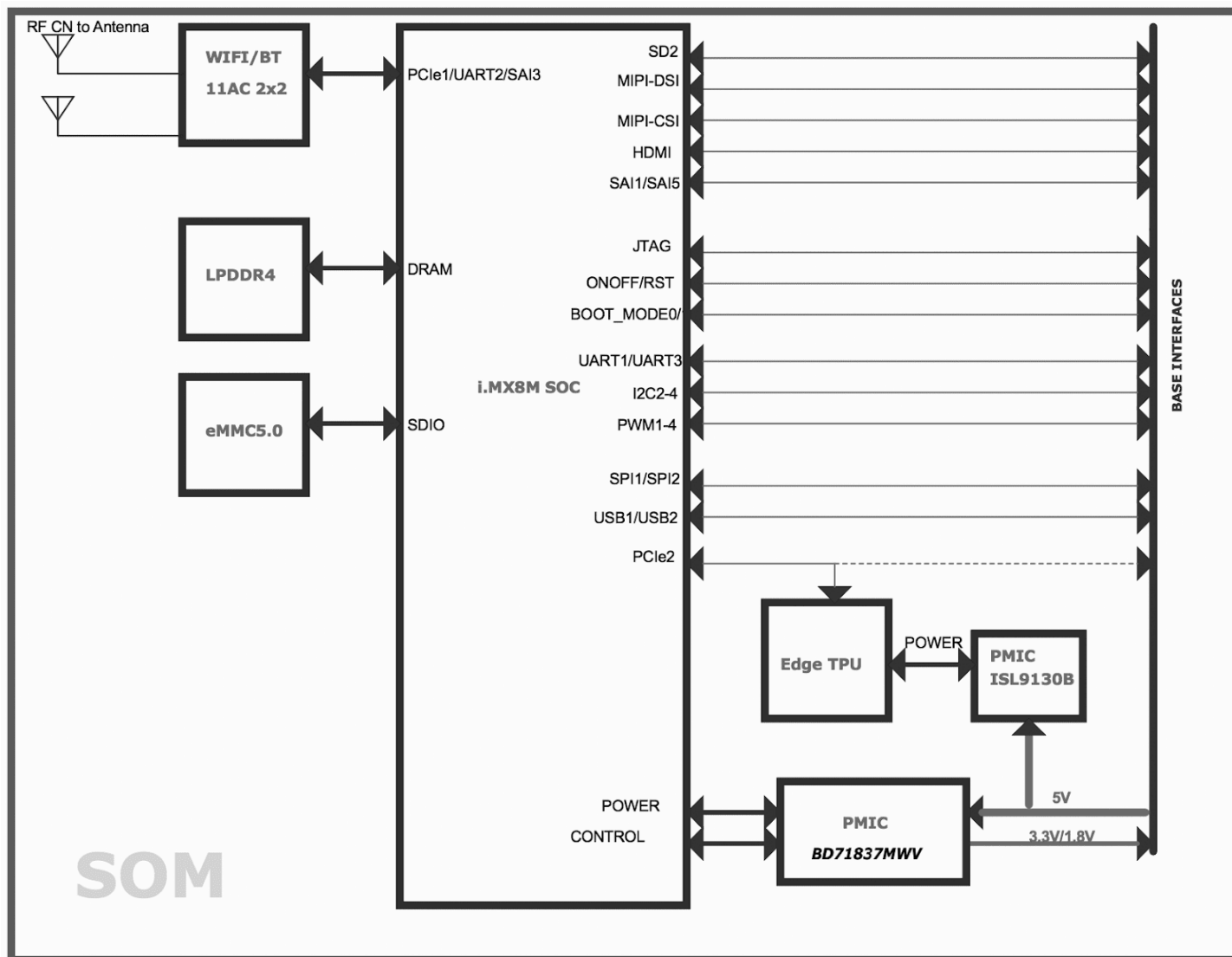
Figure 1. Block diagram of the SoM components
