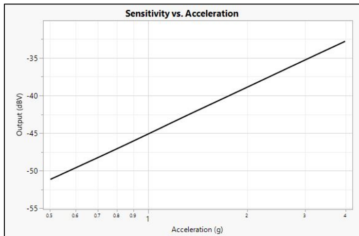
Output vs Acceleration, 250Hz
