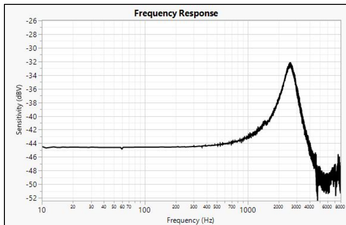
Frequency Response
