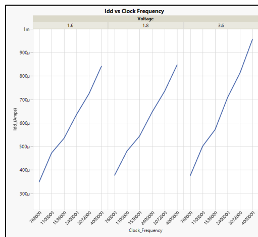
c. Idd vs Clock over Vdd
