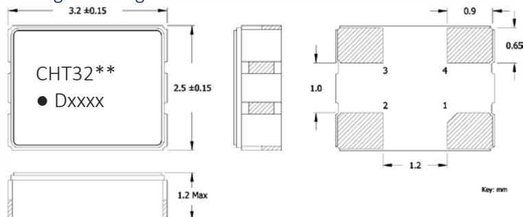
Package Drawing
