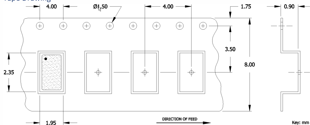
Tape Drawing
