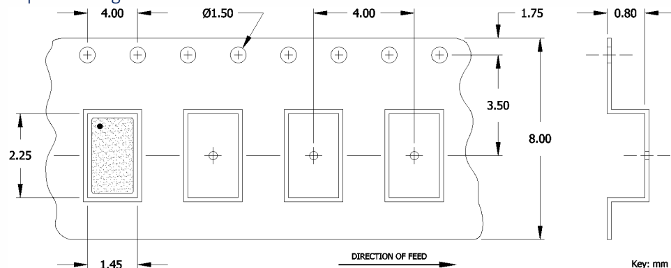
Tape Drawing
