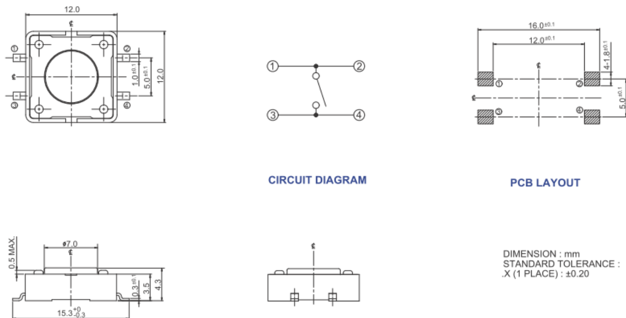
Figure 3 –224AMVC... Surface Mount Gull Wing, Actuator Height 4.3mm
