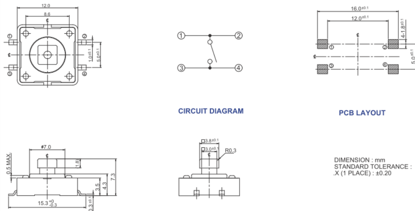
Figure 2 –224AMVB... Surface Mount Gull Wing, Actuator Height 8.5mm
