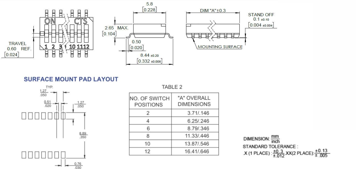
Figure 2 – Surface Mount Gull Wing Terminal
