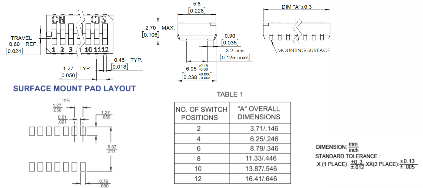
Figure 1 – Surface Mount J Bend Terminal
