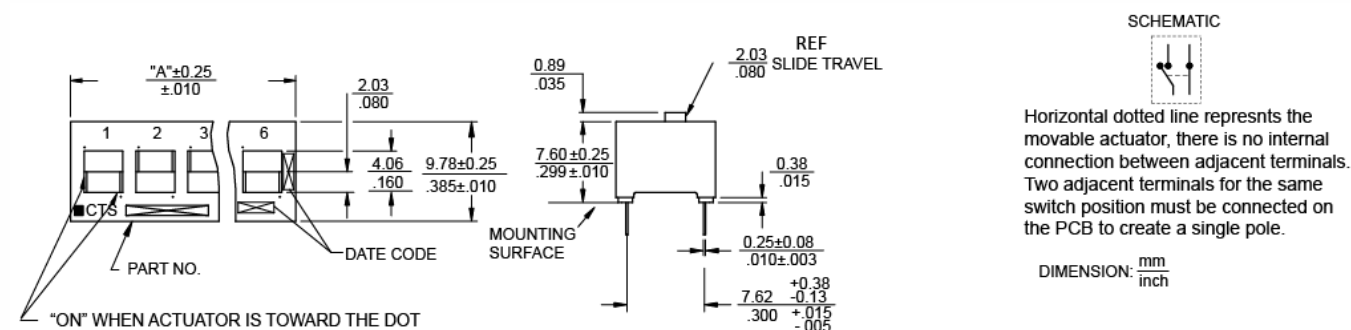
Figure 2 – SPDT
