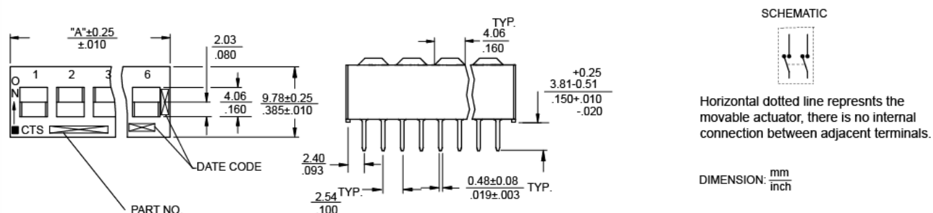
Figure 3 – DPST
