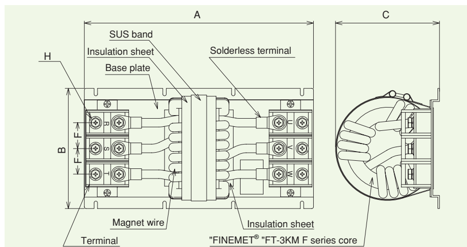
Figure 43. FN coil
