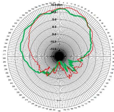
Antenna Pattern
