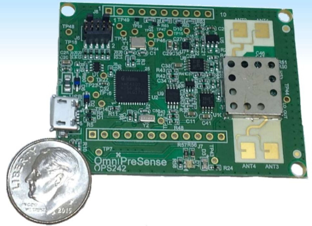
OPS242 Sensor
