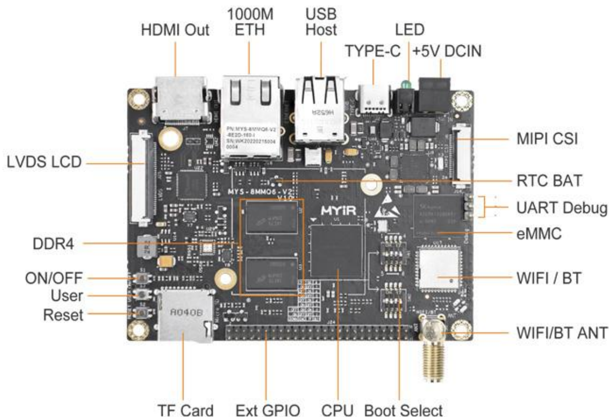
Figure 1-2 MYS-8MMX-V2 Top-View
