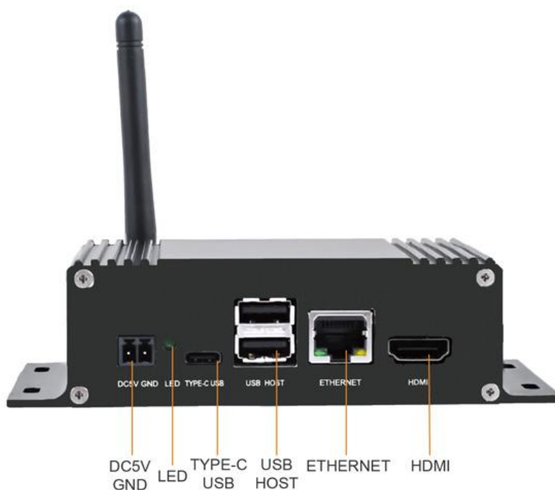
Figure 1-4 MYS-8MMX-V2 Box
