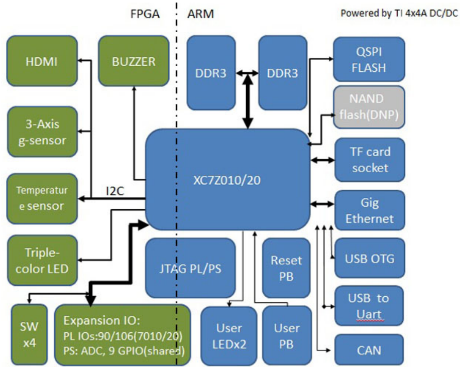
Figure 1-5 Z-turn Board Function Block Diagram
