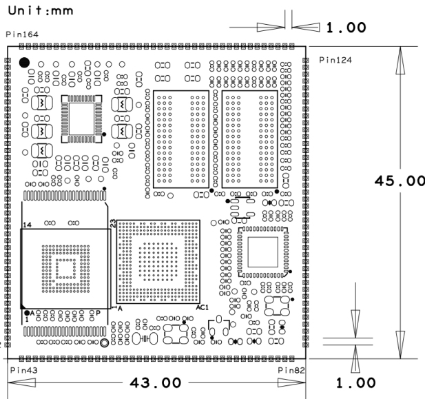
Figure 1-10 MYC-YA157C Dimensions Chart
