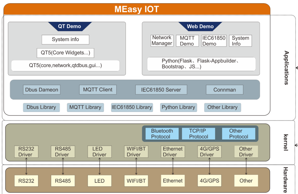
Figure 1-13 MEasy-IOT System Structure
