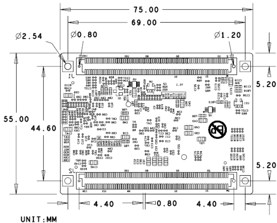
Figure 1-9 Dimensions of MYC-C7Z010/20 CPU Module
