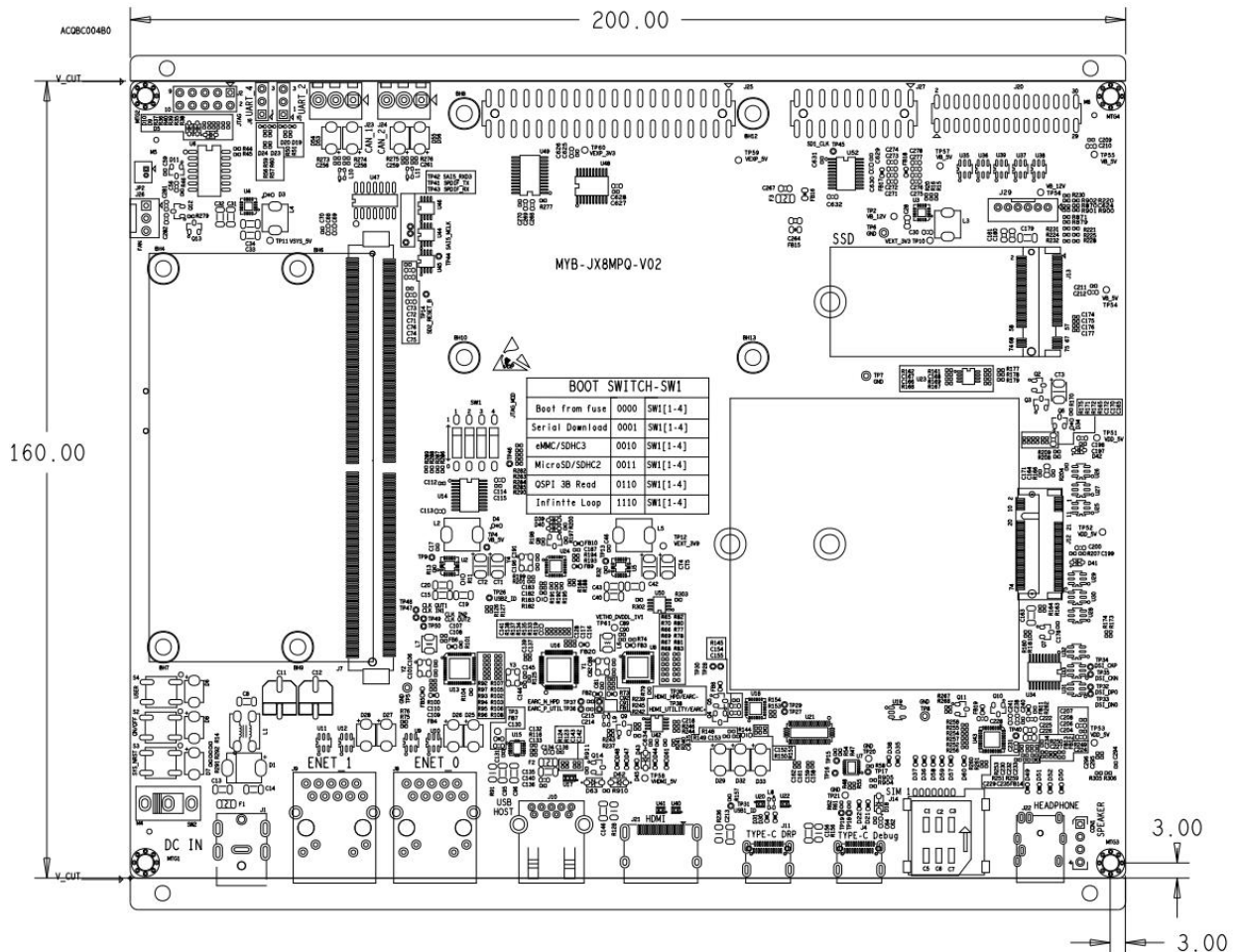
MYD-JX8MPQ Development Board Dimensions Chart
