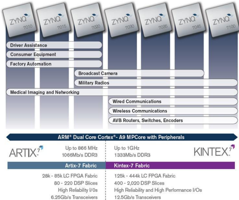
Zynq-7000 Devices
