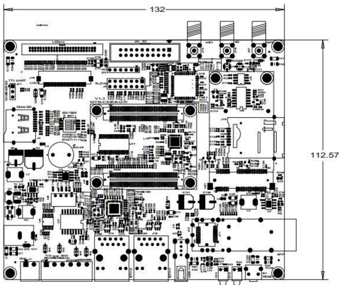
Figure 1-8 MYD-C335X-G Dimensions Chart
