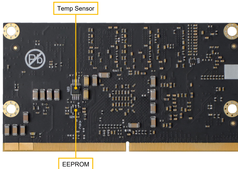
Figure 1-3 MYC-J1028X CPU Module Bottom-view
