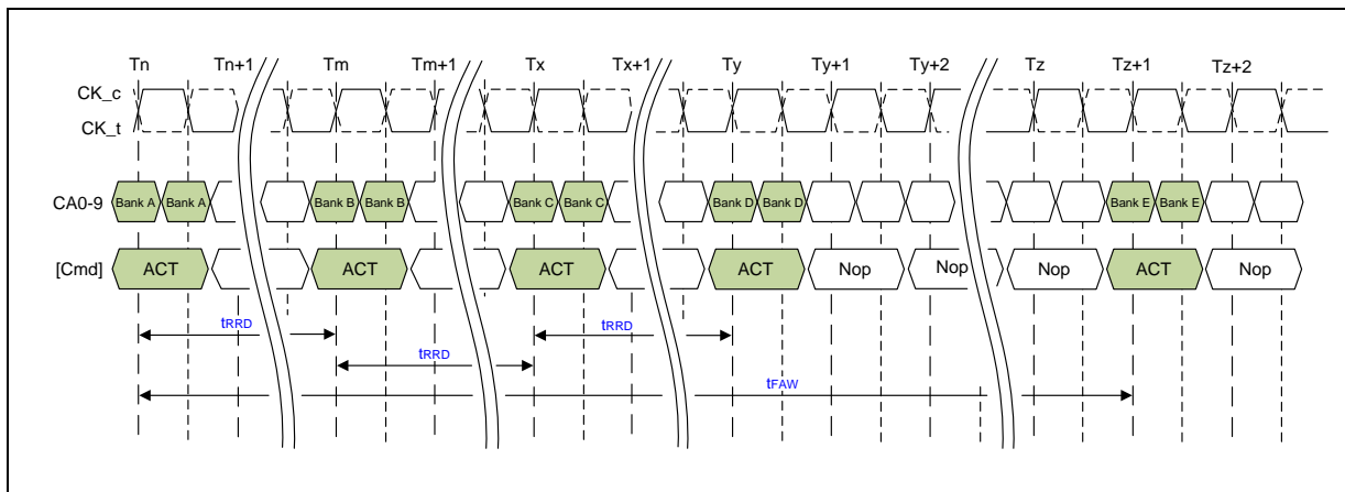
Figure 4 - tFAW Timing
