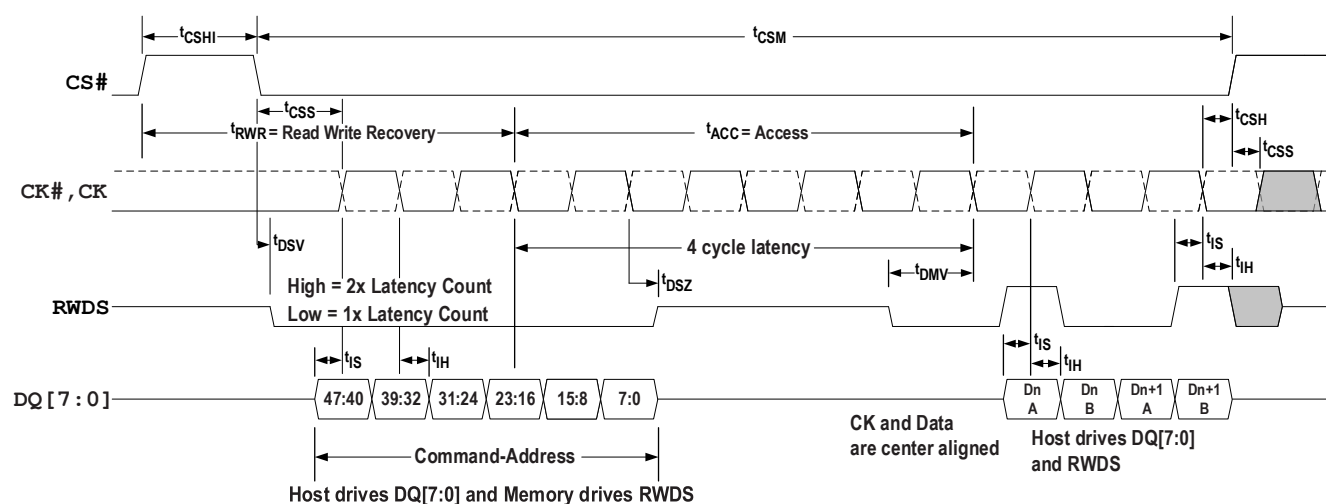
Figure 25 - Write Timing Diagram — No Additional Latency
