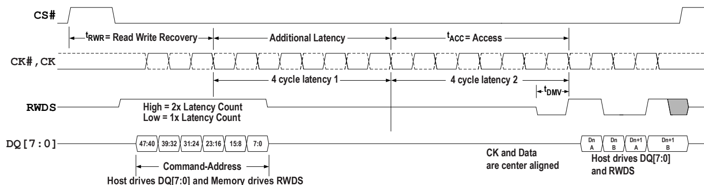
Figure 26 - Write Timing Diagram — With Additional Latency
