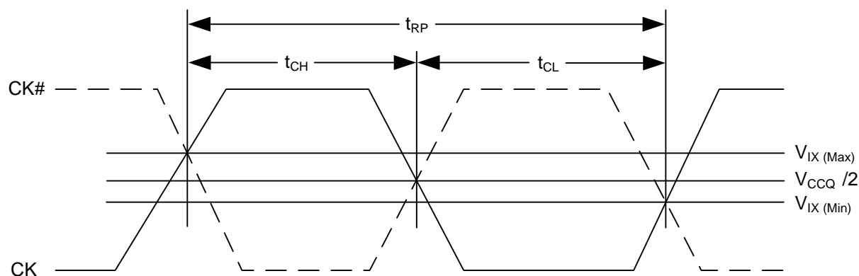
Figure 21 - Clock Characteristics
