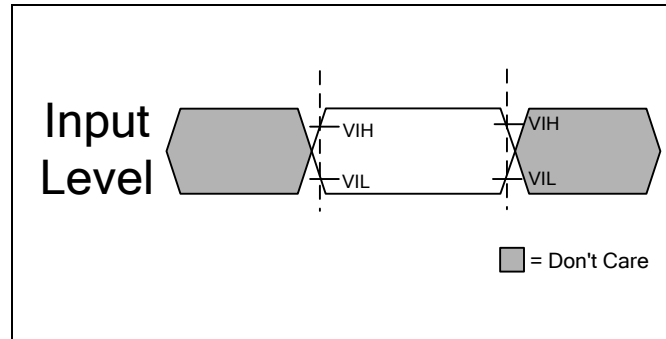
Figure 147 - LPDDR4 Input AC timing definition for Reset_n and ODT_CA
