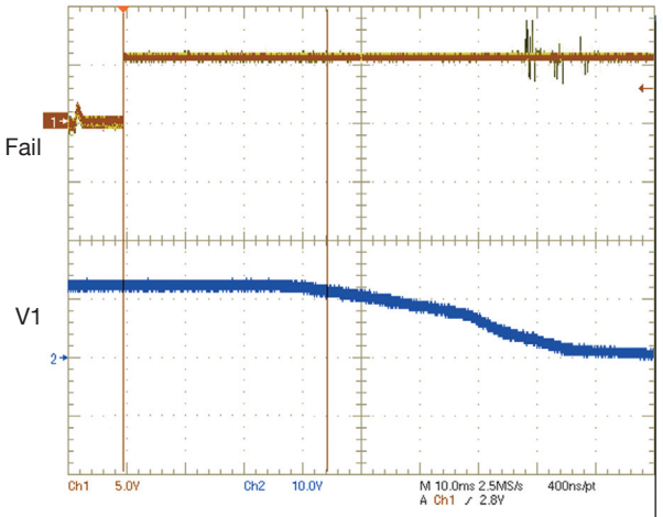
Figure 11 V1 warning time example at Power Fail signal 230 VAC 250 W load (35 ms)
