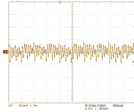
Figure 5 V1 CCM250PS24 (full load) 84 mV pk-pk ripple. 20 MHz BW
