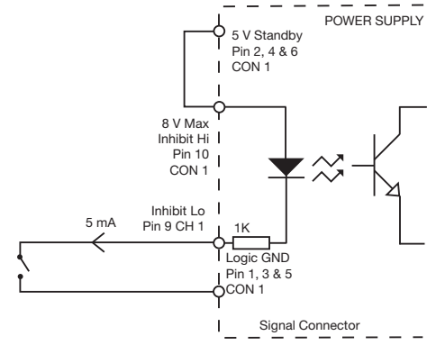
Figure 13 Inhibit (Lo)
