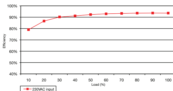
Figure 8 CCB250PS24
