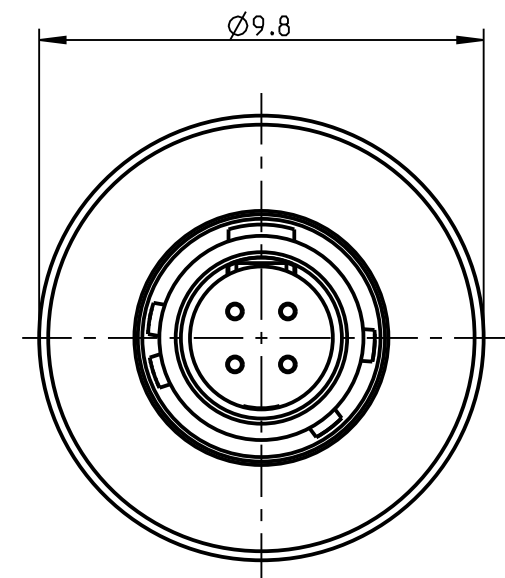
A1CWA-P04MBC0-0000 Mechanical coding: A Color coding: light brown
