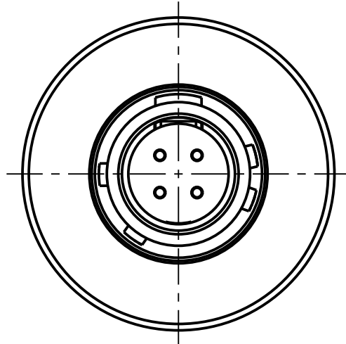
A1CWB-P04MBC0-0000 Mechanical coding: B Color coding: red
