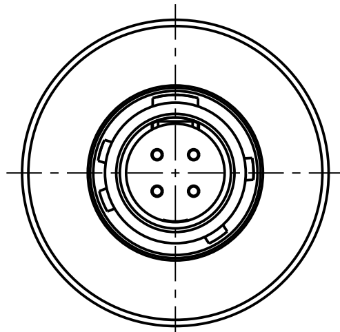
A1CWC-P04MBC0-0000 Mechanical coding: C Color coding: blue
