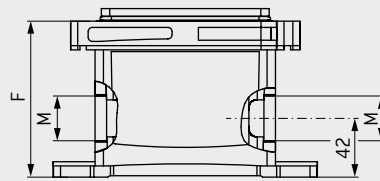
B SURFACE MOUNTED HOUSING
