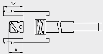
SPINDLE LOCKING
