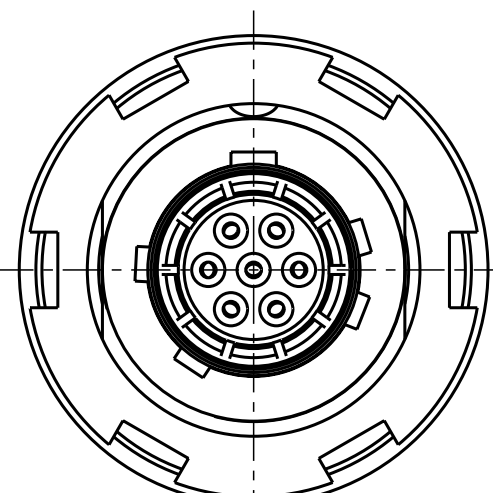
G80YCR-P07WCD0-000L Mechanical coding: C Color Coding: blue
