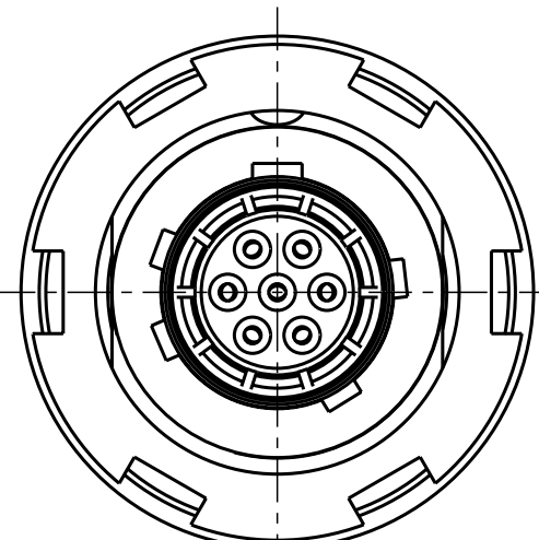
G80YDR-P07WCD0-000L Mechanical coding: D Color Coding: green
