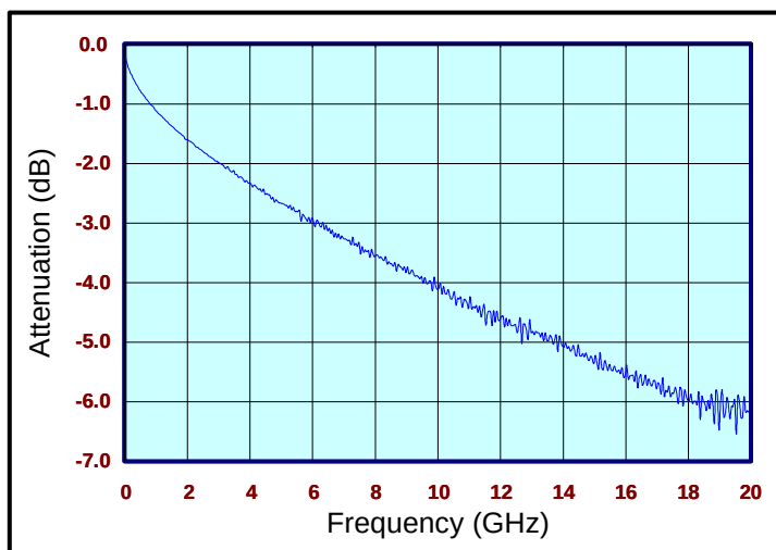
PN: CCSMA-MM-SS402-120 INSERTION LOSS (S21)
