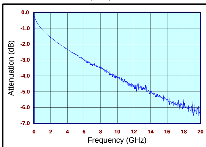
PN: CCSMA-MM-SS402-120 INSERTION LOSS (S12)
