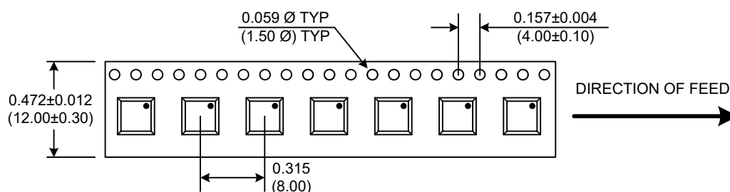
TAPE AND REEL
