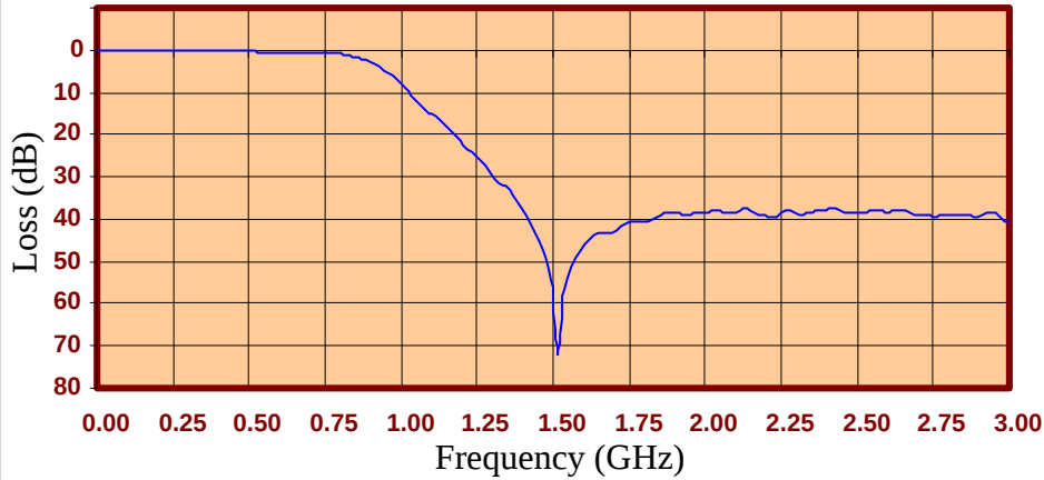
800 MHz Insertion Loss
