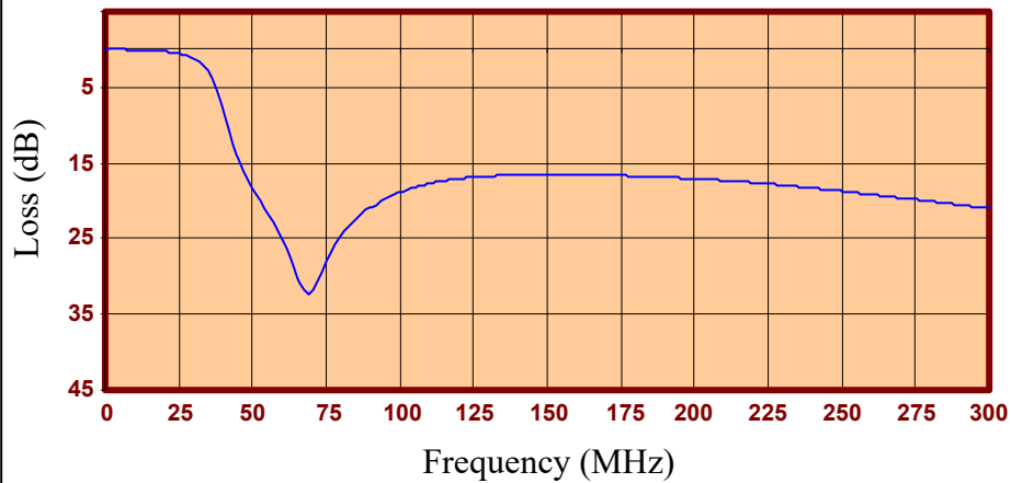
Return Loss
